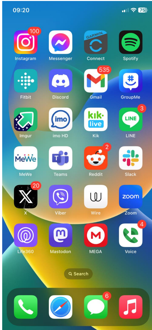
Figure 3 – Home screen 2
