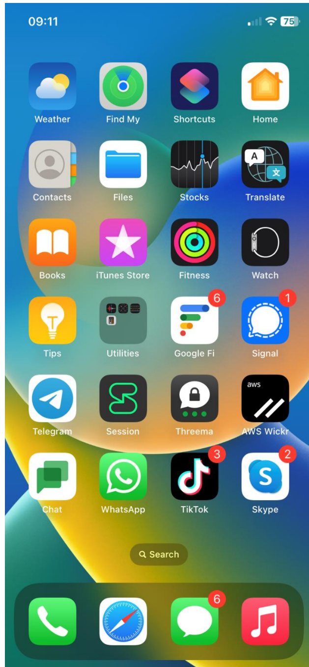
Figure 2 - Home screen 1
