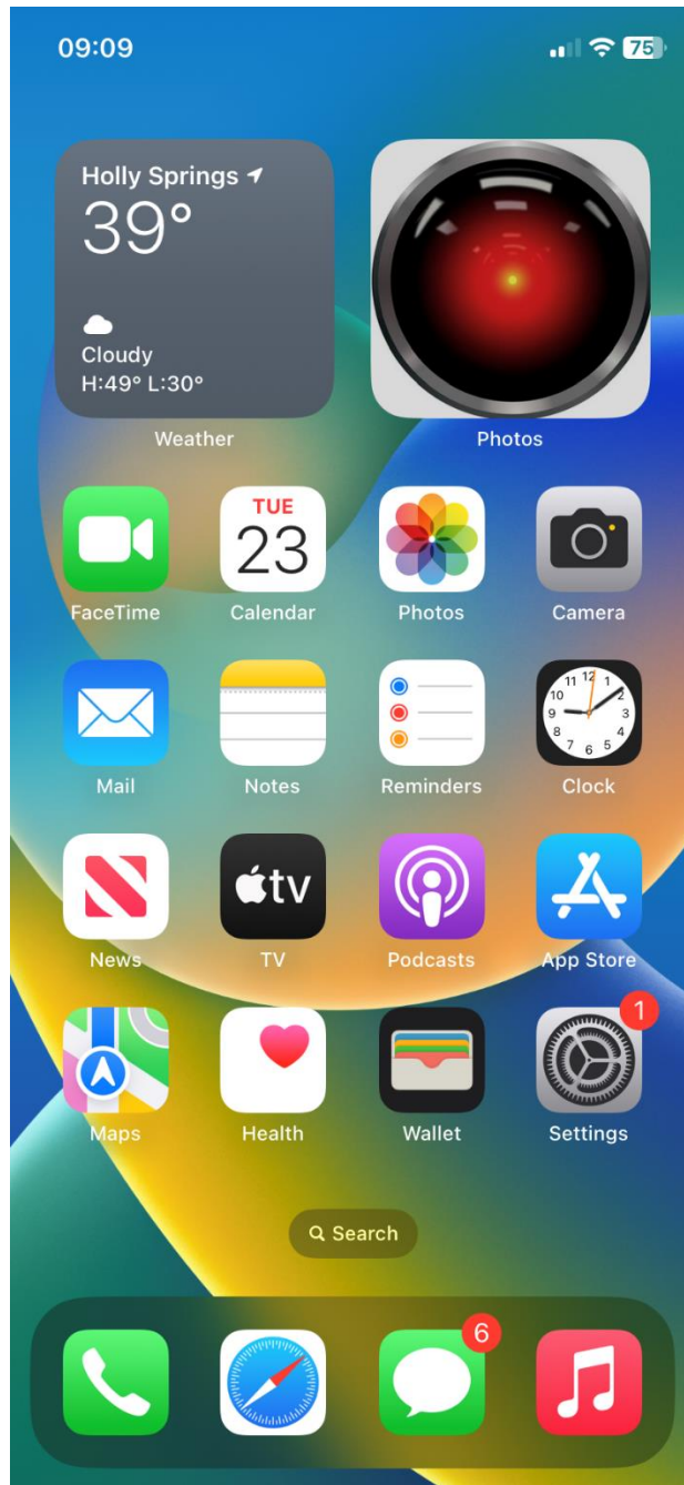
Figure 1 - Home screen
