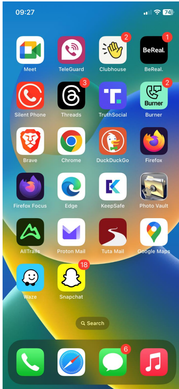
Figure 4 – Home screen 3
